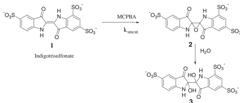
Scheme 1. Oxidation of indigo blue with MCPBA.
