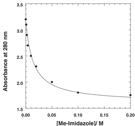
Fig. 3. A plot of the absorbance at 280 nm of MCPBA/1-MeImidazole solutions as a function of [\text{1-MeImidazole}] at [\text{MCPBA}]_{\text{T}} = 0.5 \text{ mM} in \text{MeOH}/\text{H}_2\text{O} (8:2) at 25 °C. The solid line is the calculated absorbance using Eq. 6a with the values of K , \epsilon_1 , and \epsilon_2 given in Table 1.
