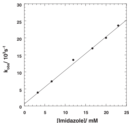
Fig. 4. A plot of the observed-first-order rate constant with [imidazole] for the reaction of MCPBA (2.0 mM) and indigo blue (0.05 mM) in MeOH/H 2 O (8:2) at 25 °C.
