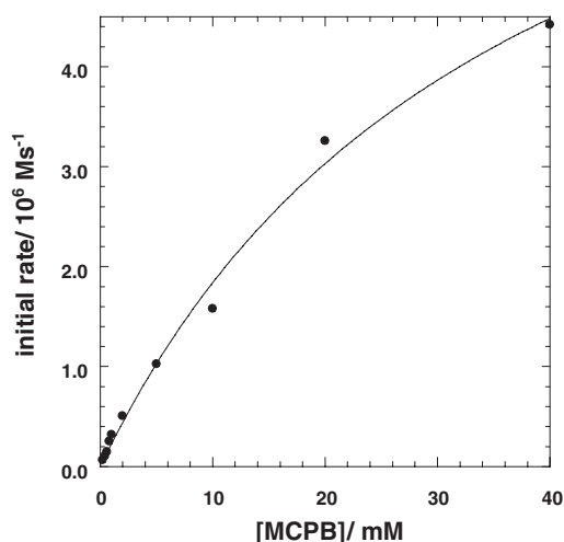
Fig. 6. Variation of the initial rate with [MCPBA] for the reaction of MCPBA and indigo blue (0.05 mM) in the presence of imidazole (20 mM) in MeOH/H 2 O (8:2) at 25 °C. The solid line represents the calculated initial rate using Eq. 8 with the values of k_1 = 0.025 \text{ M}^{-1} \text{ s}^{-1} , k_{-1} = 3.2 \times 10^{-4} \text{ s}^{-1} , and k_2 = 7.1 \text{ M}^{-1} \text{ s}^{-1} .
