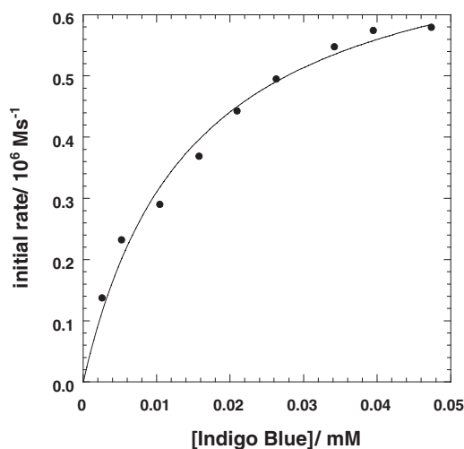
Fig. 5. Variation of the initial rate with [indigo blue] for the reaction of MCPBA (1.0 mM) and indigo blue in the presence of imidazole (20 mM) in MeOH/H 2 O (8:2) at 25 °C. The solid line represents the calculated initial rate using Eq. 8 with the values of k_1 , k_{-1} , and k_2 given in Table 2.
