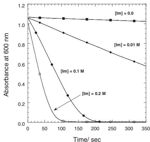
Fig. 1. The absorbance–time curves for the oxidation of indigo blue (0.05 mM) with MCPBA (2.0 mM) in the presence and absence of imidazole. The absorbance change was recorded at 600 nm due to the loss of indigo dye ( \epsilon_{600} = 1.9 \times 10^4 \text{ M}^{-1} \text{ cm}^{-1} ) in \text{CH}_3\text{OH}/\text{H}_2\text{O} (8:2) at 25 °C.
