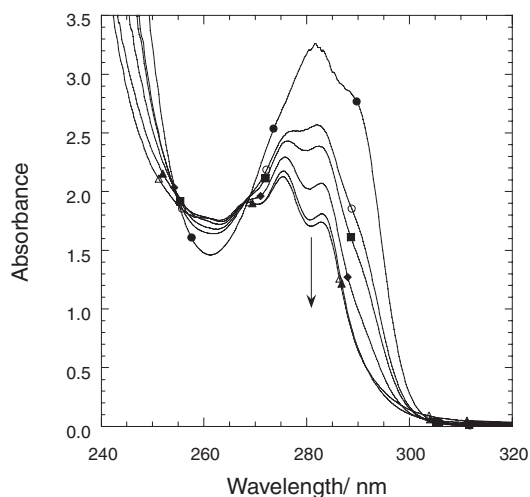
Fig. 2. UV spectra of equilibrated MCPBA/1-MeImidazole mixtures in \text{CH}_3\text{OH}/\text{H}_2\text{O} (8:2) at 25 °C. The total MCPBA concentration is 0.5 mM. Reading downward at 282 nm, the 1-MeImidazole concentrations are 0.0 (●), 10 (○), 20 (■), 50 (◆), 100 (▲), 200 (△) mM. Approximate isosbestic point at 269 nm.
