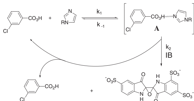
Scheme 2. A reaction scheme for the oxidation of indigo blue with MCPBA as catalyzed by imidazole.
