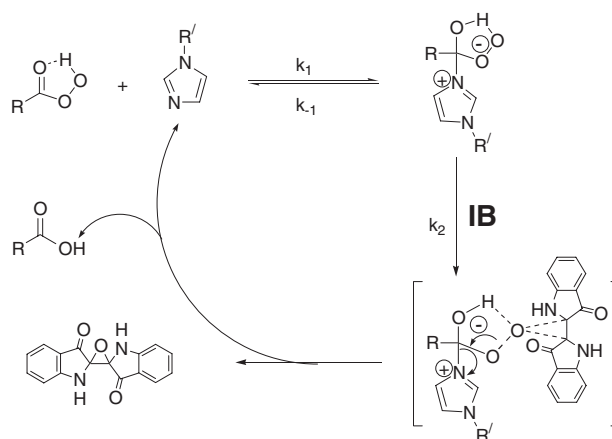
Scheme 3. A suggested mechanism for the oxidation of an olefin by MCPBA/imidazole.
